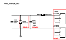
Motor Contact
