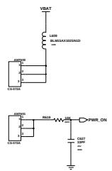
Power Key
