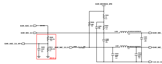
Ear MIC
