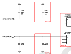
SPK Contact
